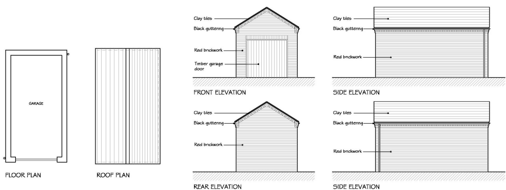
REAR ELEVATION
